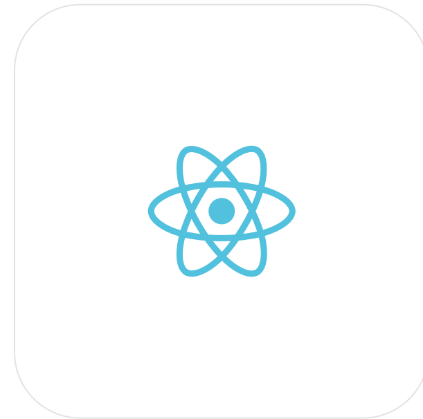
React Native
