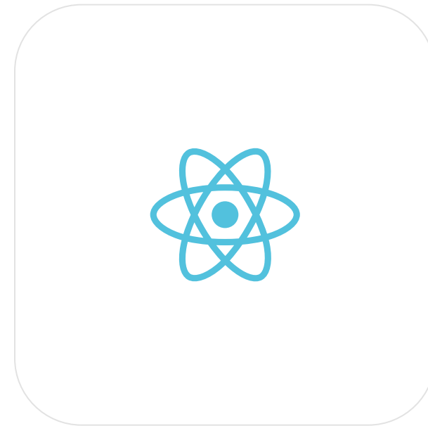
React
